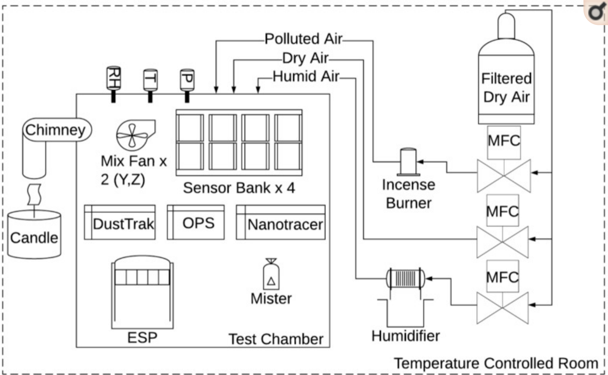
Schematic showing the arrangement of the test chamber and the supporting equipment (image reprinted under the terms and conditions of the Creative Commons Attribution (CC BY 4.0) license—License MDPI, Basel, Switzerland Sensors 2020, 20, 2219; doi:10.3390/s20082219).
